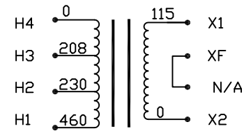
INTERNALLY JUMPERED TO FUSE TERMINAL CONNECTION DIAGRAM
