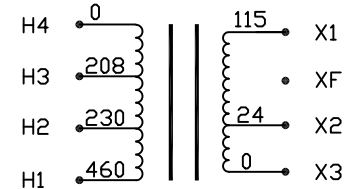
CONNECTION DIAGRAM
