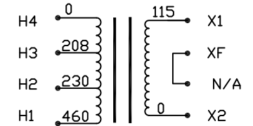
INTERNALLY JUMPERED TO FUSE TERMINAL CONNECTION DIAGRAM
