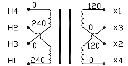
CONNECTION DIAGRAM
