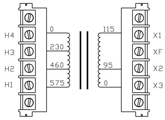
CONNECTION DIAGRAM
