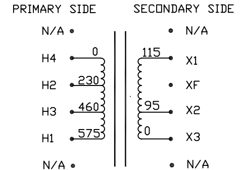
CONNECTION DIAGRAM
