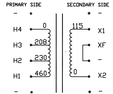
INTERNALLY JUMPERED TO FUSE TERMINAL CONNECTION DIAGRAM
